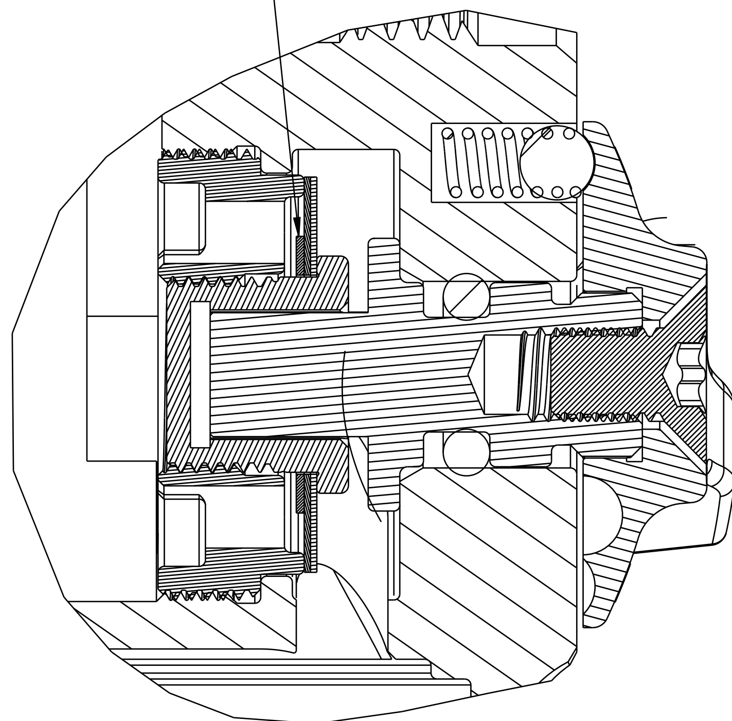
SECTION A-A SCALE 8:1
