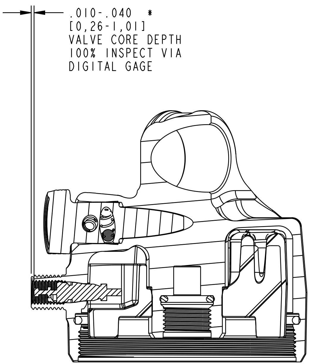
SECTION B-B
