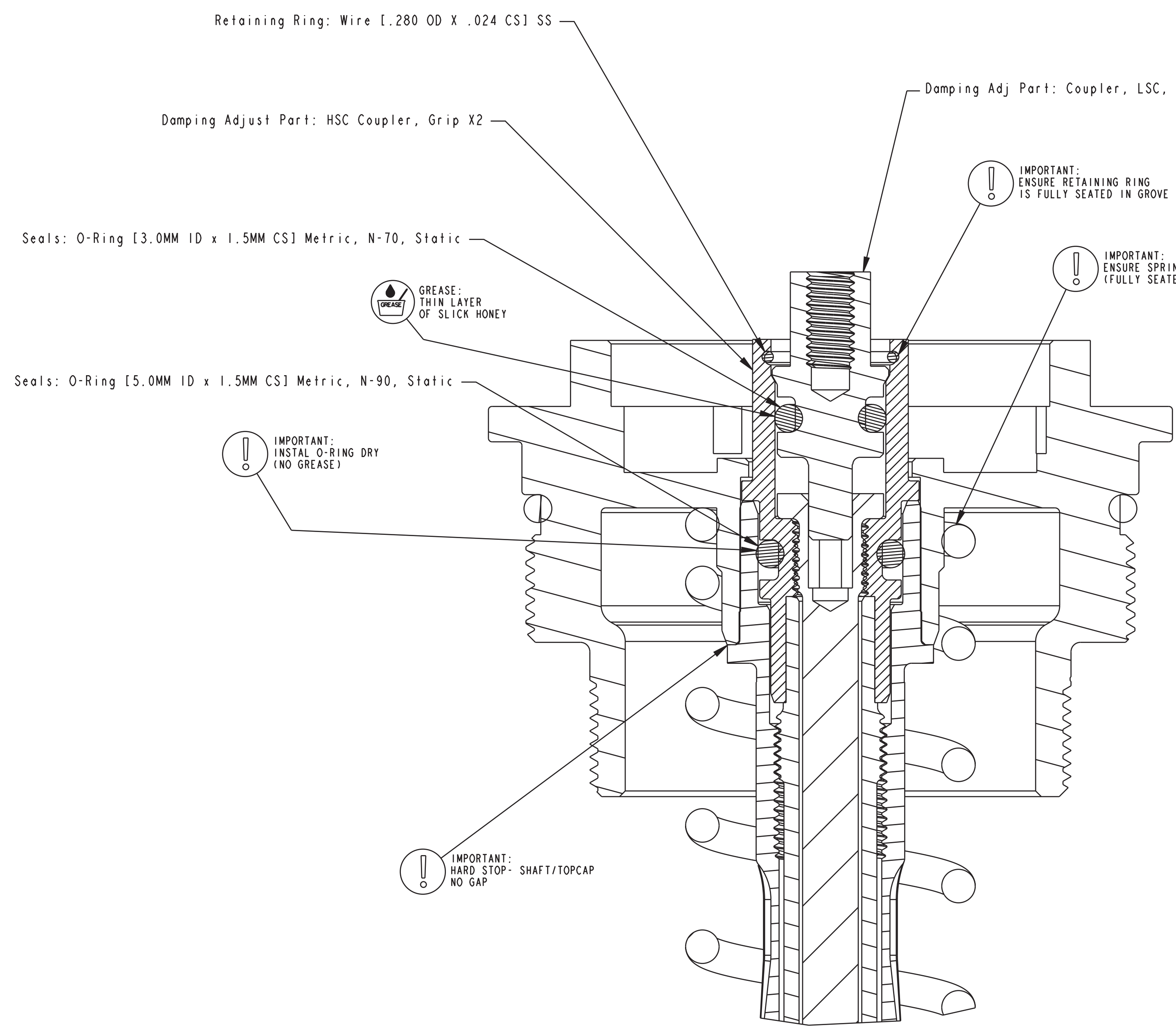
DETAIL Z SCALE 6:1
