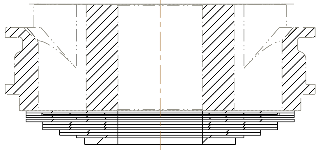
SECTION A-A SCALE 6:1
