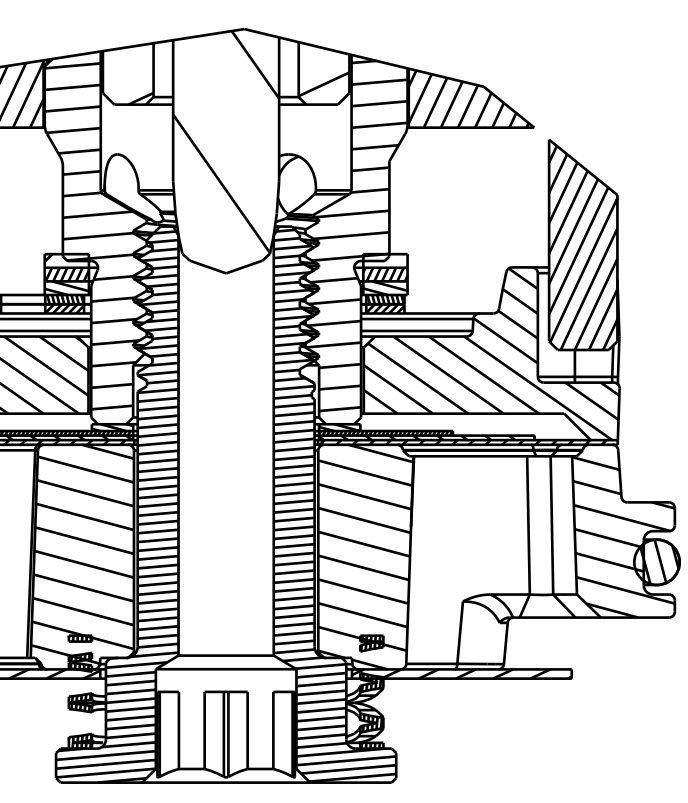
DETAIL C SCALE 6:1
